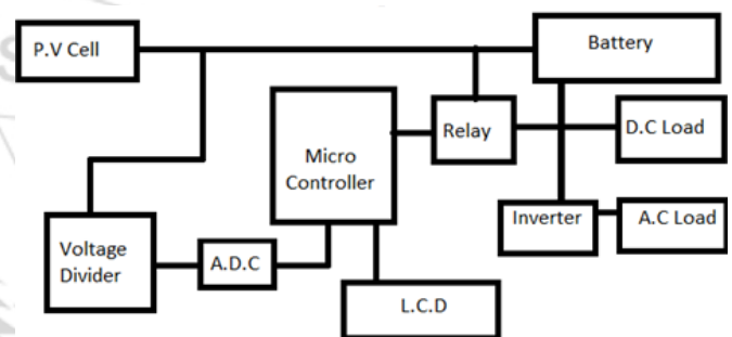
Figure 1.1: Block diagram
