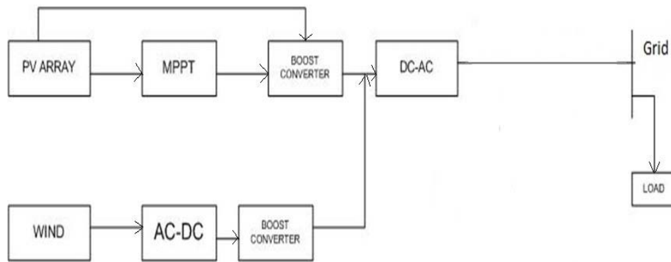
Figure 1: Grid Connected PV-Wind Hybrid System
